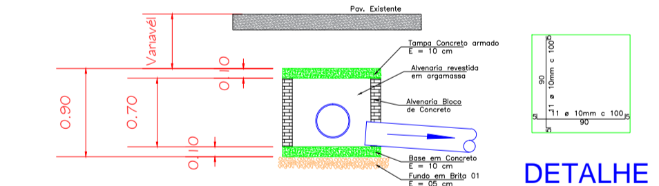
DETALHE CL 100x100/80 ESC. 1:50
