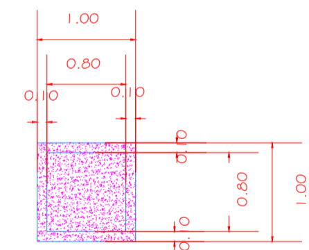
PLANTA CL 100x100/80 ESC. 1:50
