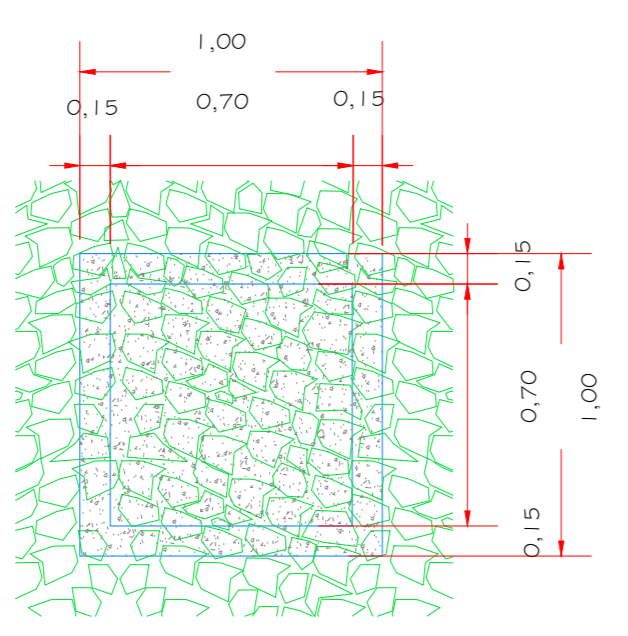
PLANTA CP01-100x100/80 ESC. 1:25
