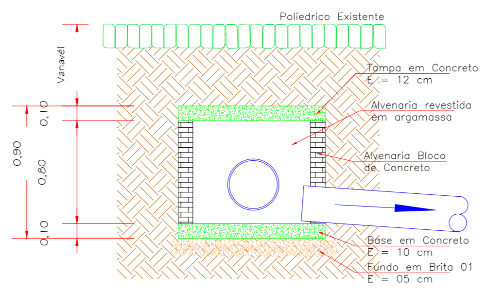
CORTE CP01-100x100/80 ESC. 1:25
