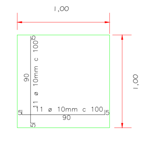
DETALHE CP01-100x100/80 ESC. 1:25
